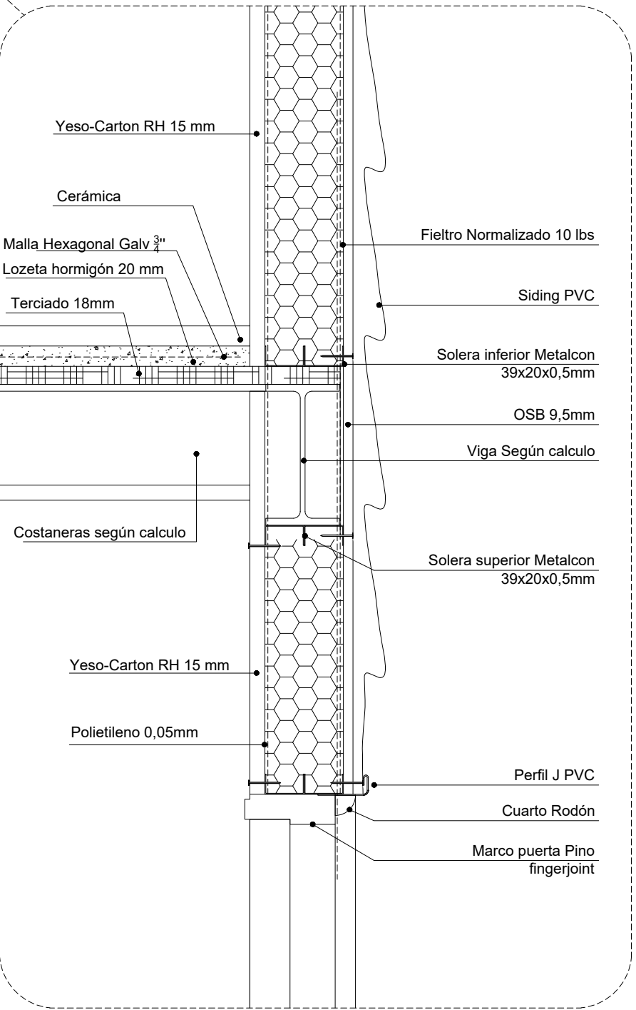
D3- Muro Perimetral F-15
